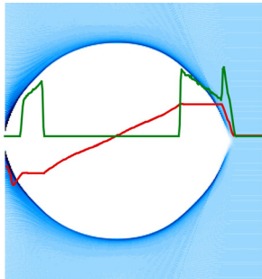
Figure 1: The longitudinal profiles (green curve) of the drive and main beams and the longitudinal wakefield (red curve) produced by these beams. The blue and white background are plasma and the ion channel, respectively.
