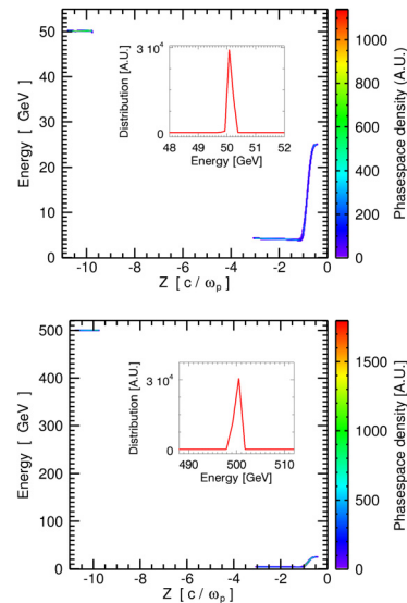
Figure 3: Phase space of the drive and main beams at the end of the acceleration in the 25 GeV (upper plot) and 475 GeV (lower plot) PWFA stages. The insets are the energy spectra of the main beams after acceleration. The FWHMs of the spectra are estimated to be 0.4% and 0.3%, respectively.
