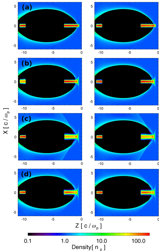
Figure 2: Beam and plasma density at four different locations in 25 GeV (left column) and 475 GeV (right column) PWFA-LC stages. (a) propagation distance s = 0\text{m} ; (b) s = 0.2\text{ m} ; (c) s = 0.38\text{ m} ; (d) s = 0.59\text{ m} . Beams are shown in red, plasma and ion channel are shown in blue and black, respectively.
