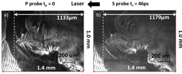
Figure 4: Two-frame interferogram at different times. a) shows P probe. b) shows S probe with 46ps delay. White dashed line shows the instantaneous position of the overdense plasma layer pushed by the radiation pressure.
