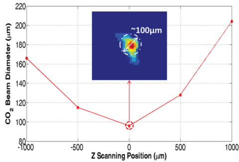
Figure 2: Spot size measurement of 10 \mu\text{m} CO 2 laser beam.
