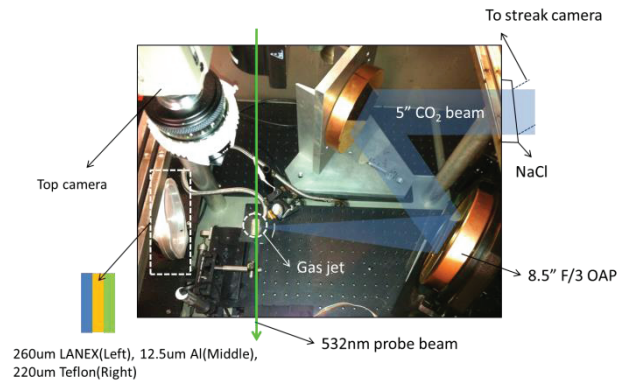
Figure 1: Experimental setup in the target chamber.
