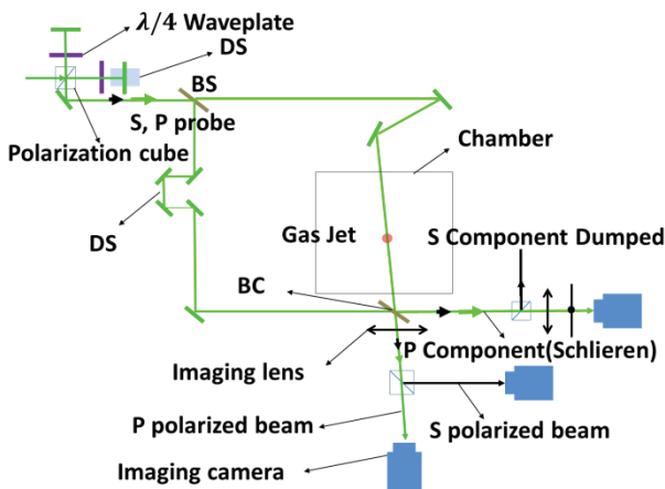
Figure 3: Schematic of the 1ps, 532nm two-frame interferometry and Schlieren diagnostics setup. Beam Splitter (BS), Delay Stage (DS), Beam Combiner (BC).
