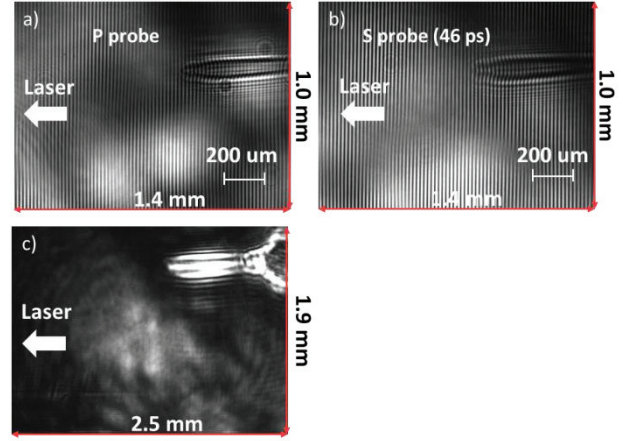
Figure 5: Two-frame interferogram and dark field schlieren images. a) Shows the channel formation as seen by P probing arm. b) Shows the channel expansion probed by S arm (46ps later). c) Shows the schlieren image for P polarized probe with a larger field of view.
